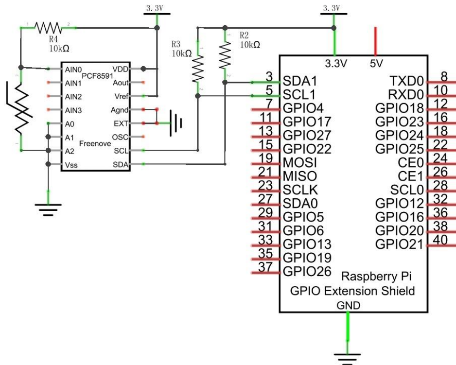
Schematic diagram
