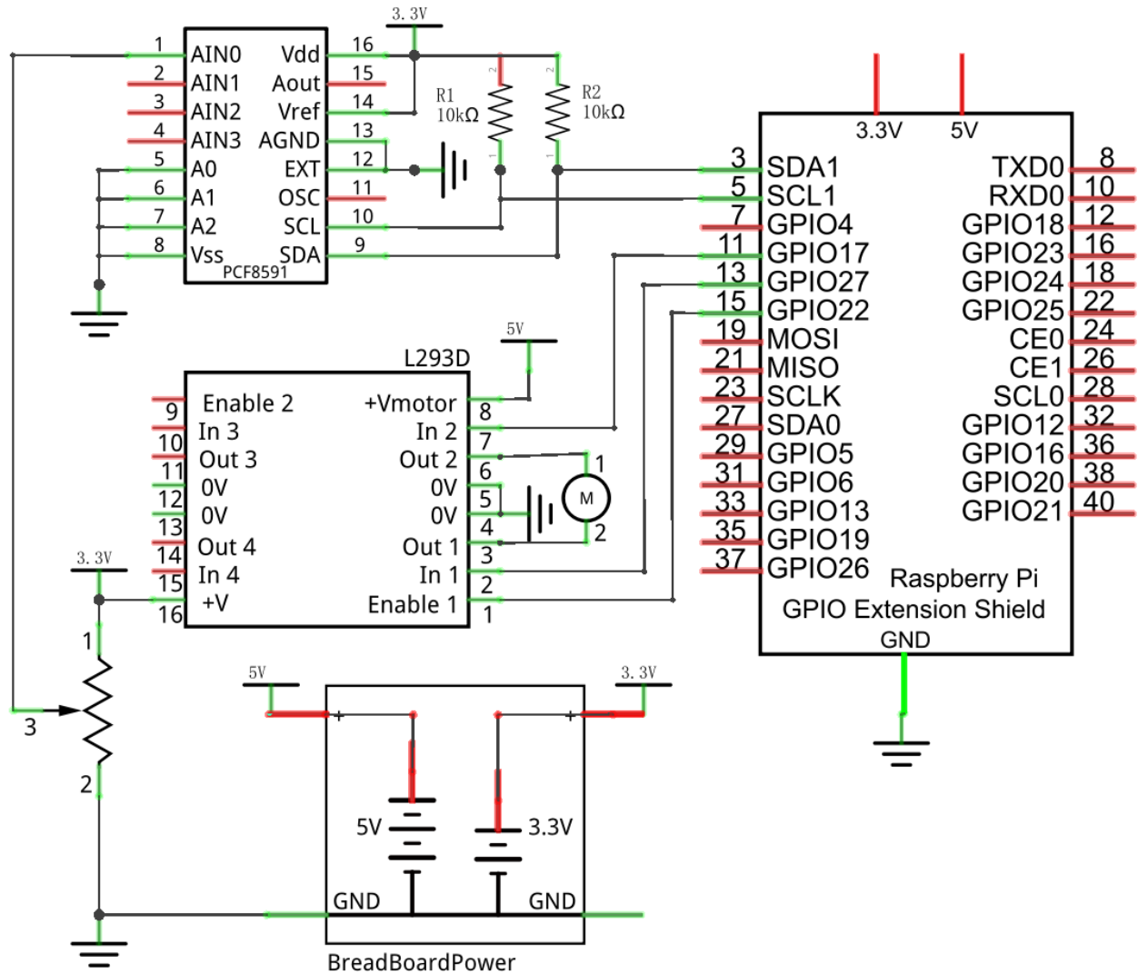
Schematic diagram
