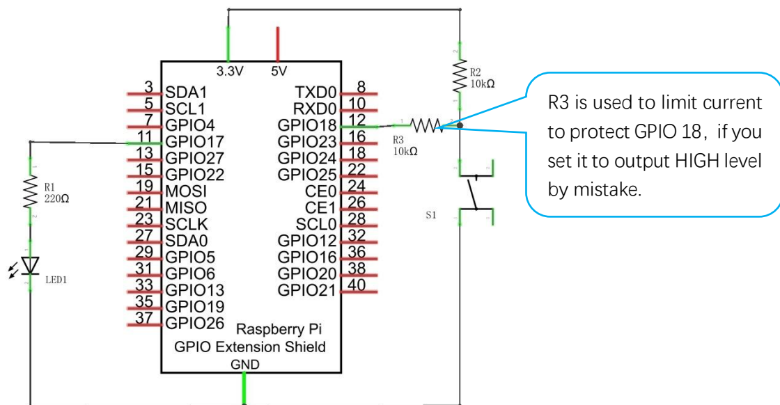
Schematic diagram
