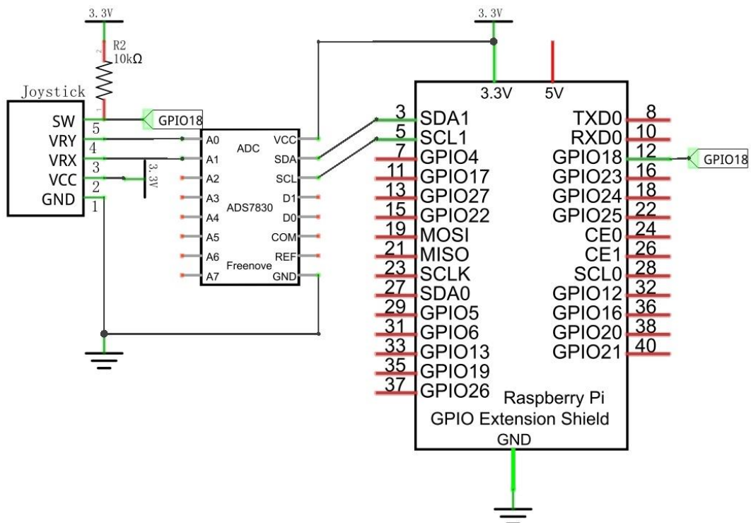
Schematic diagram
