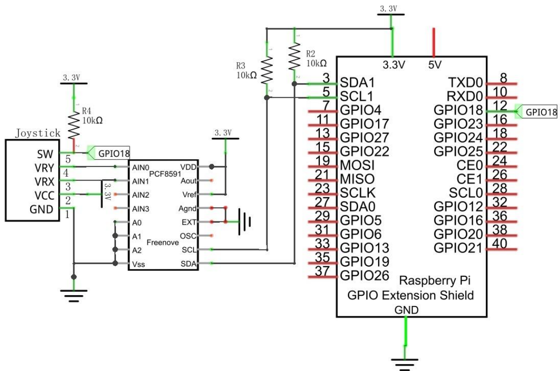
Schematic diagram
