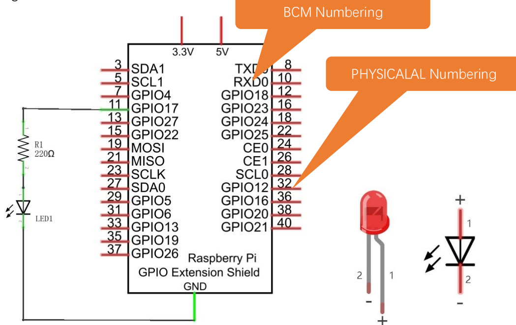
Hardware connection.
