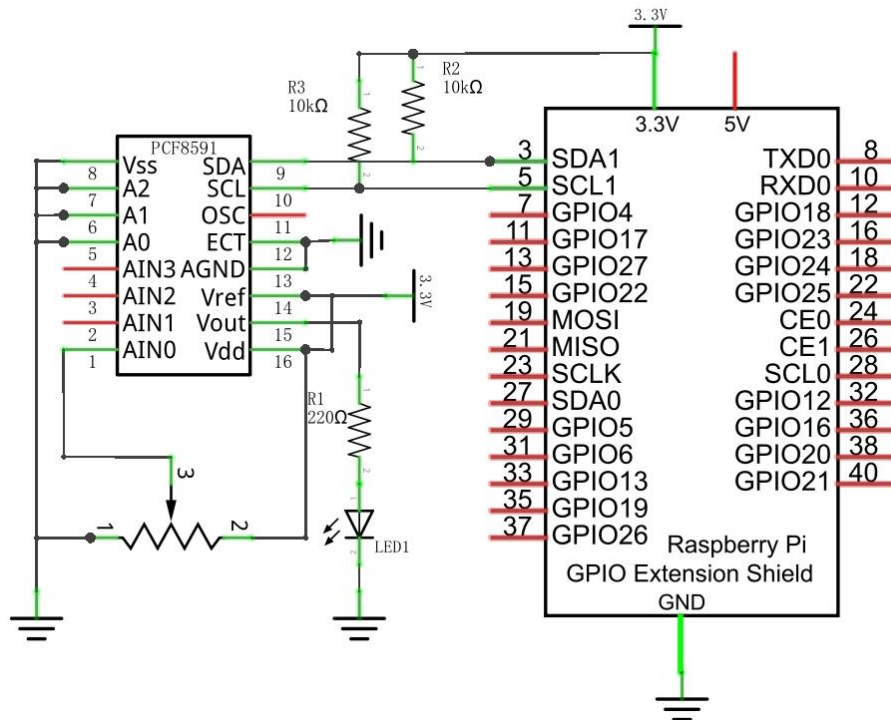
Hardware connection
