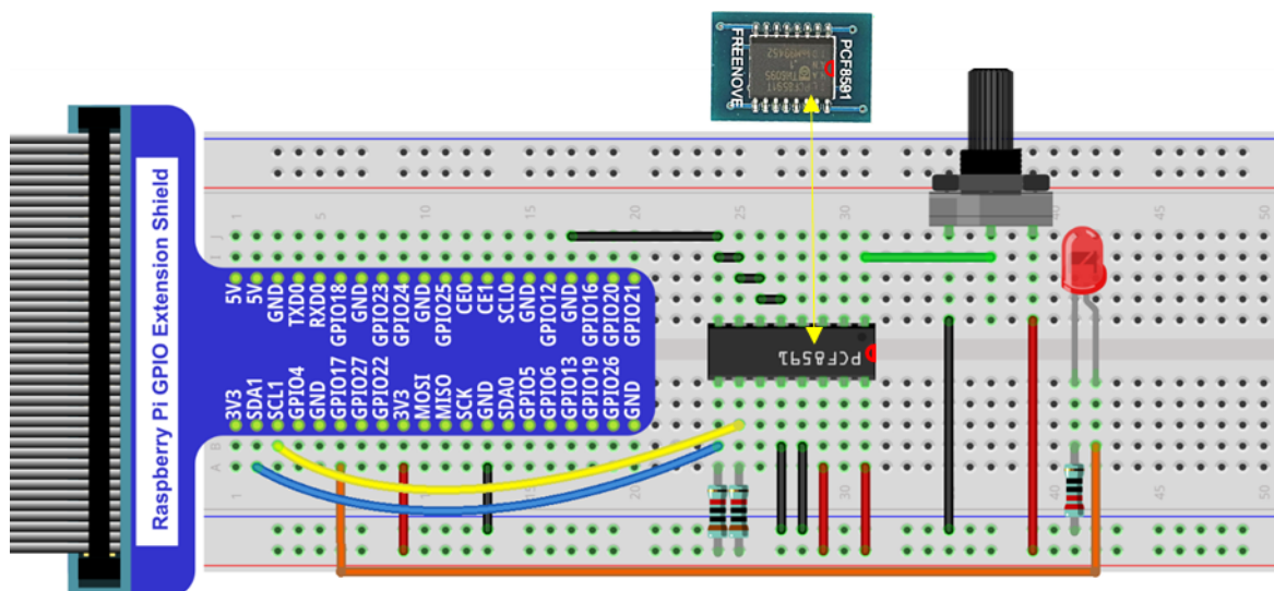
Hardware connection
