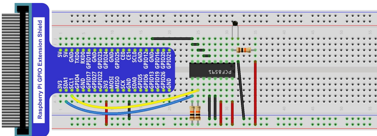
Hardware connection
