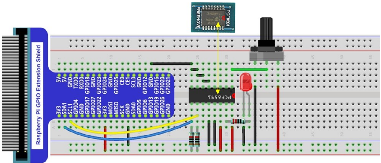
Hardware connection
