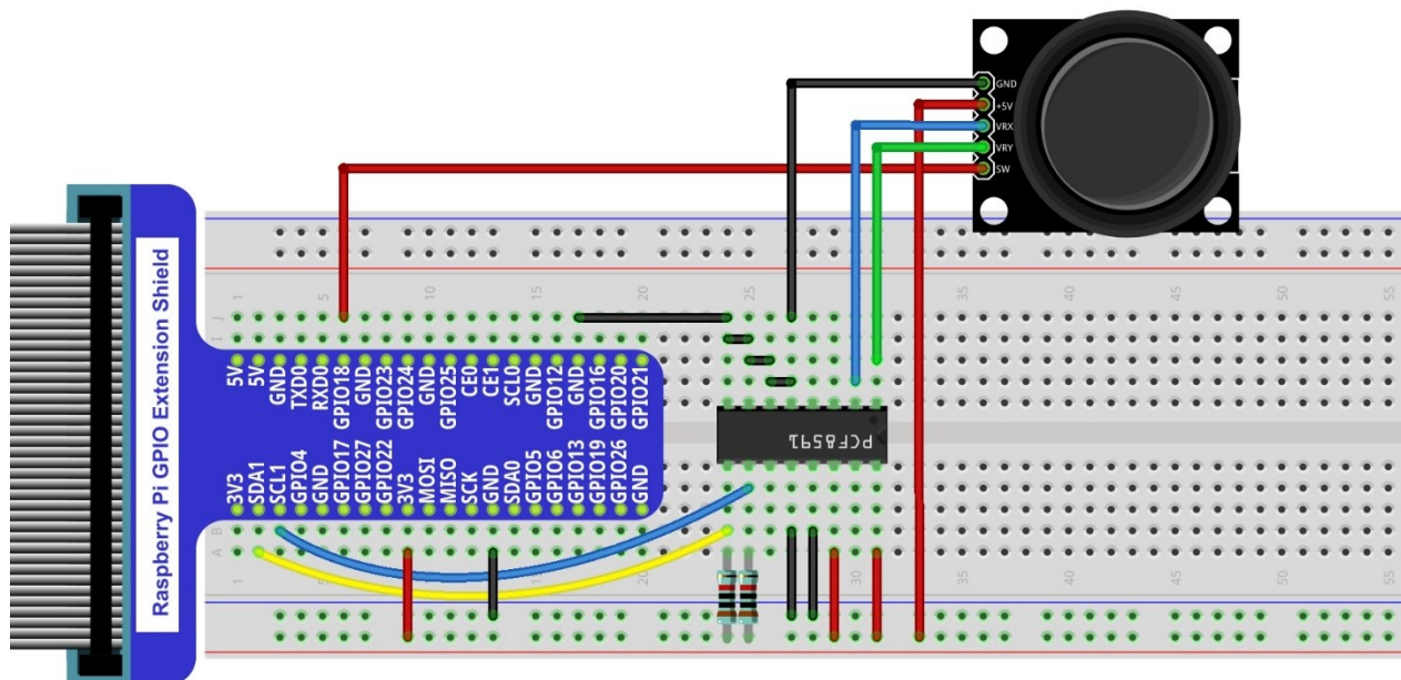
Hardware connection
