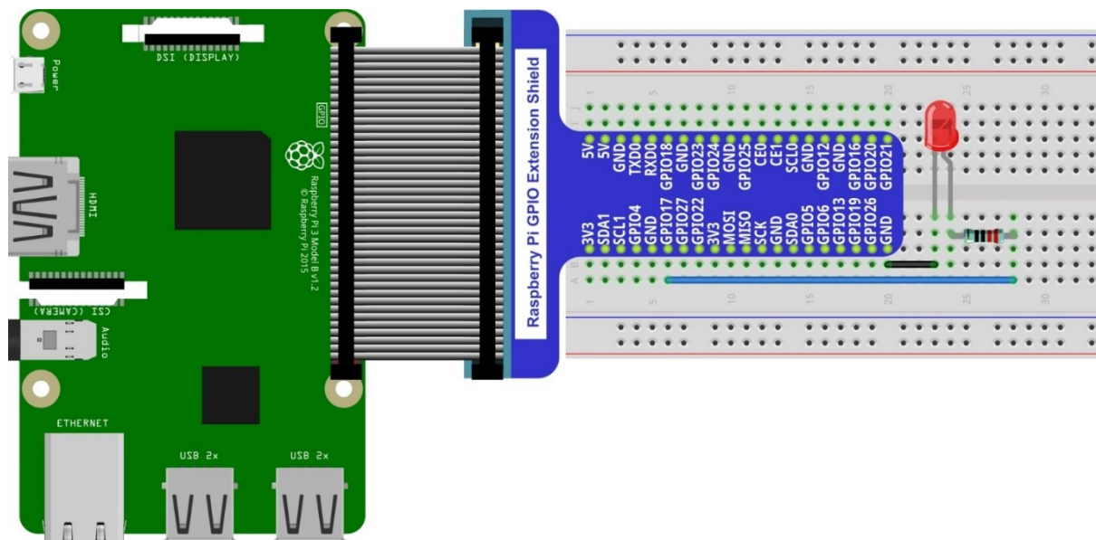
Hardware connection
