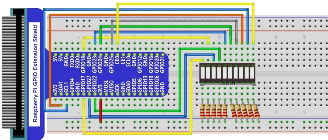
Hardware connection
