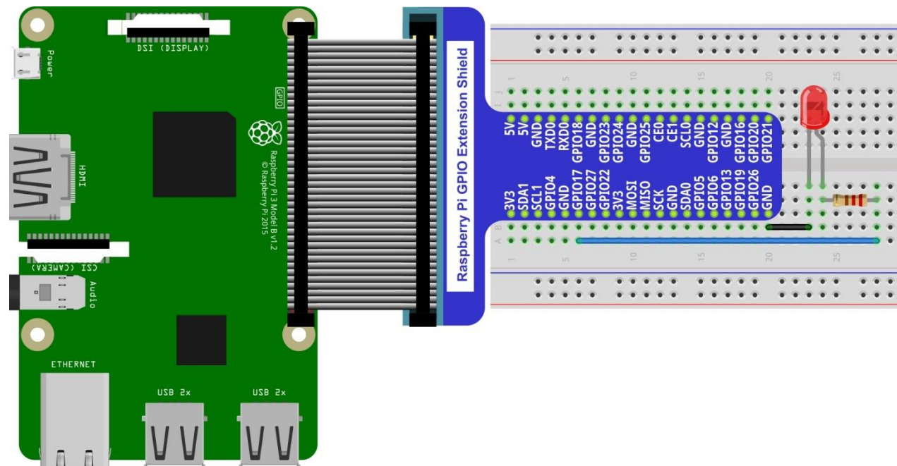
Hardware connection
