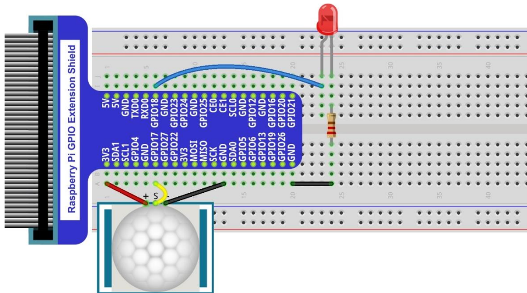
Hardware connection
