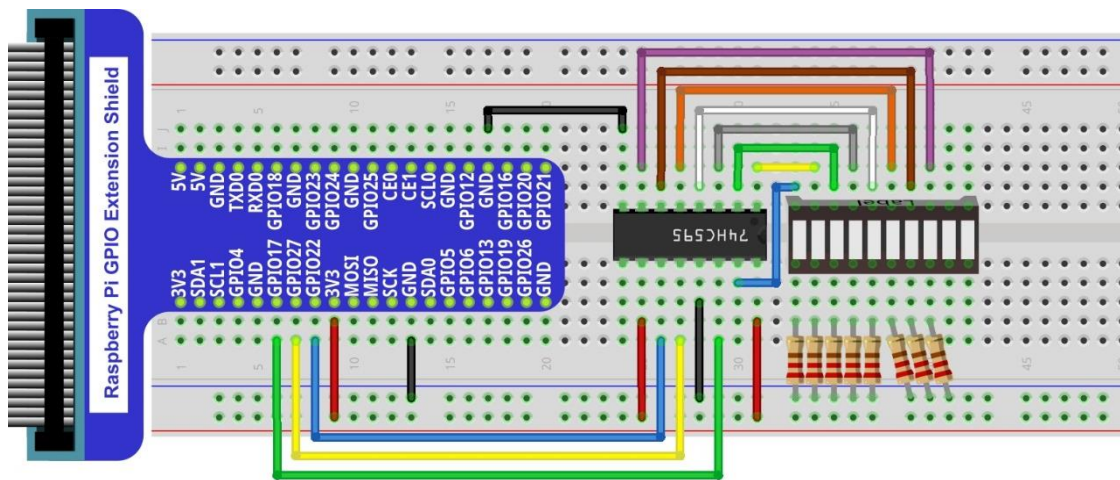
Hardware connection
