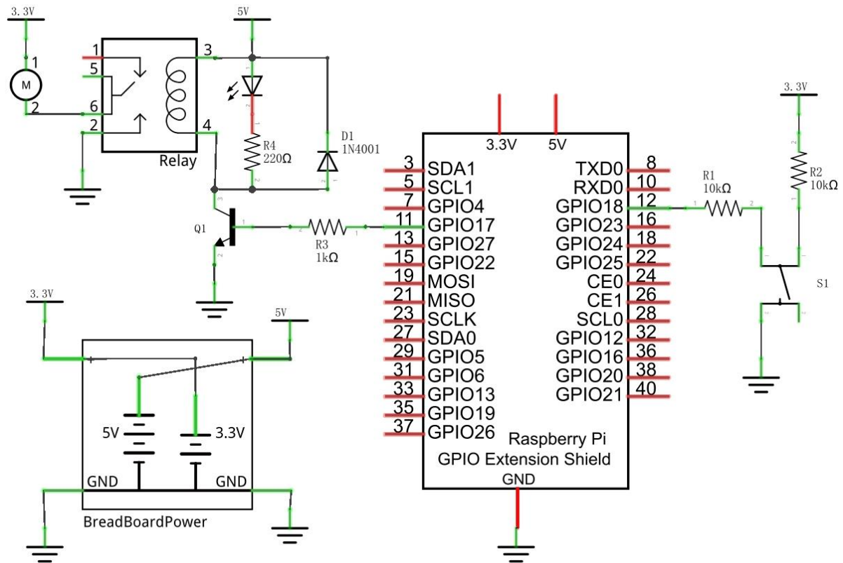
Schematic diagram
