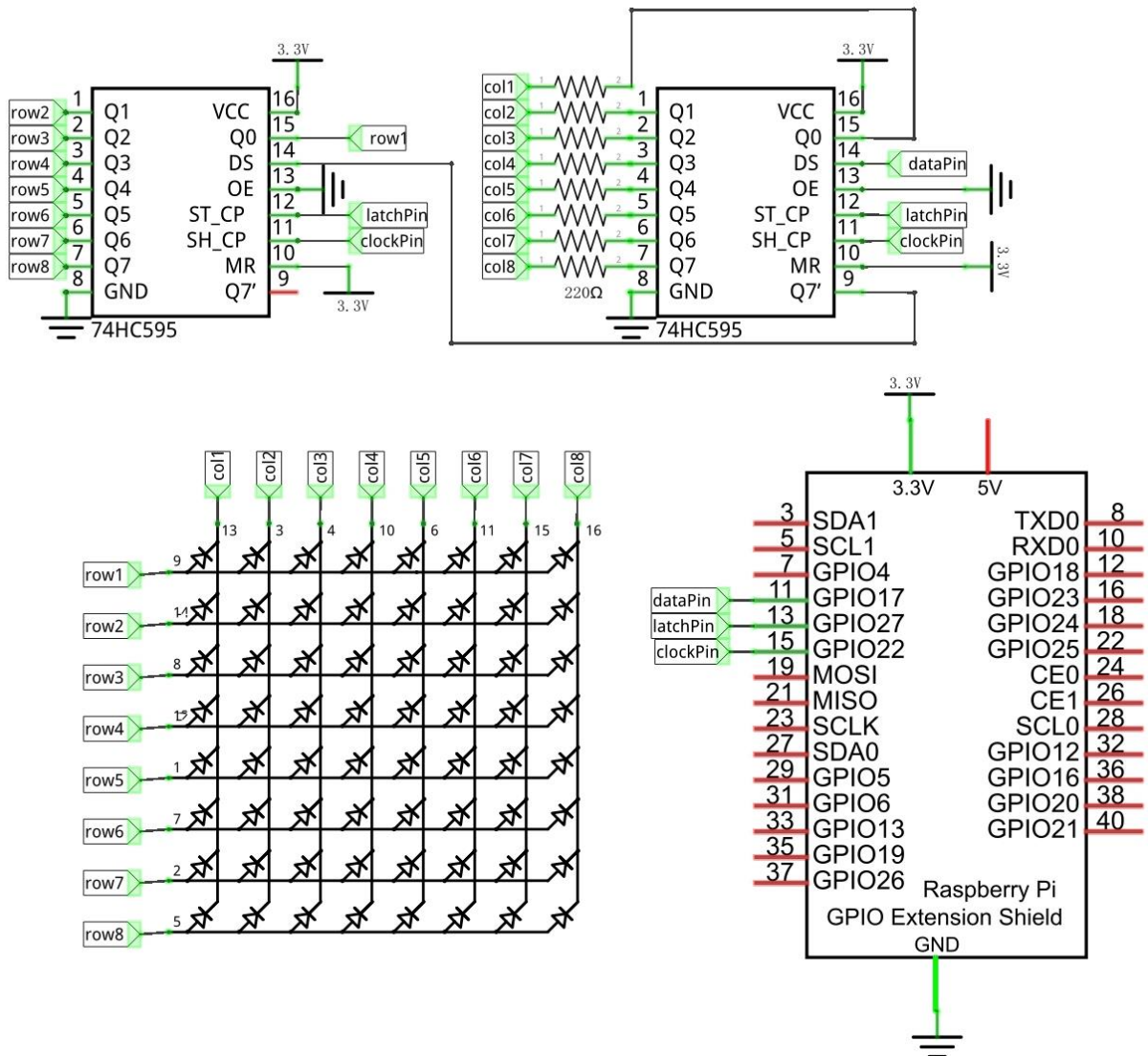
Schematic diagram
