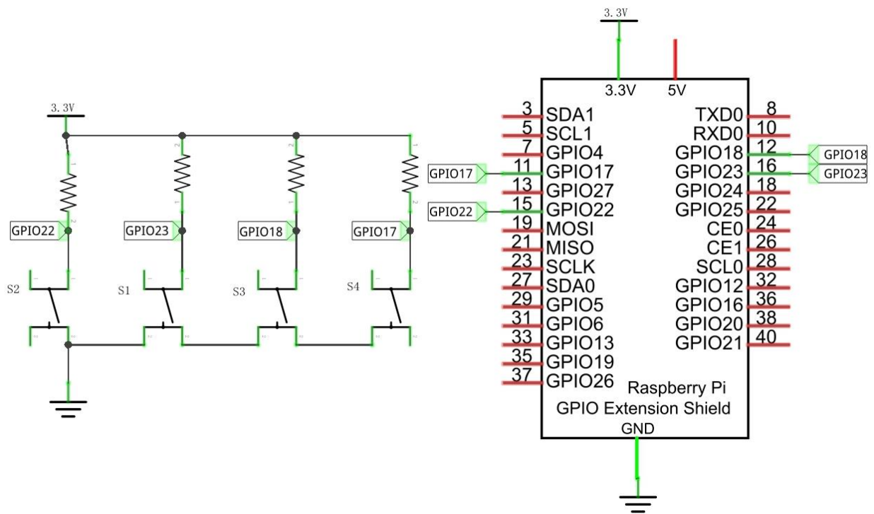
Hardware connection
