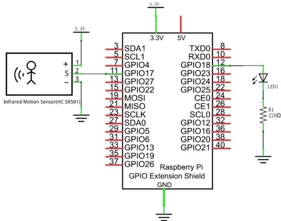
Hardware connection
