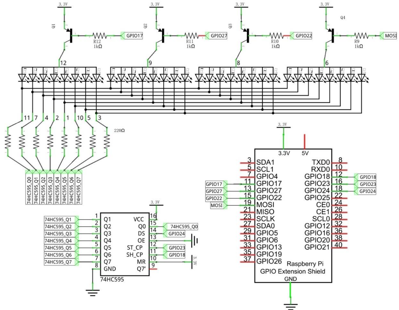
Schematic diagram
