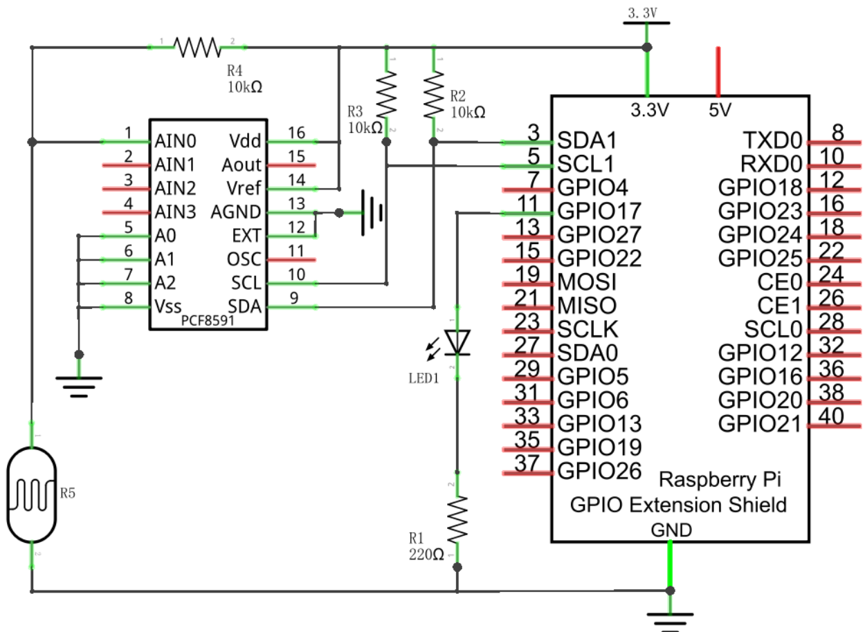
Hardware connection
