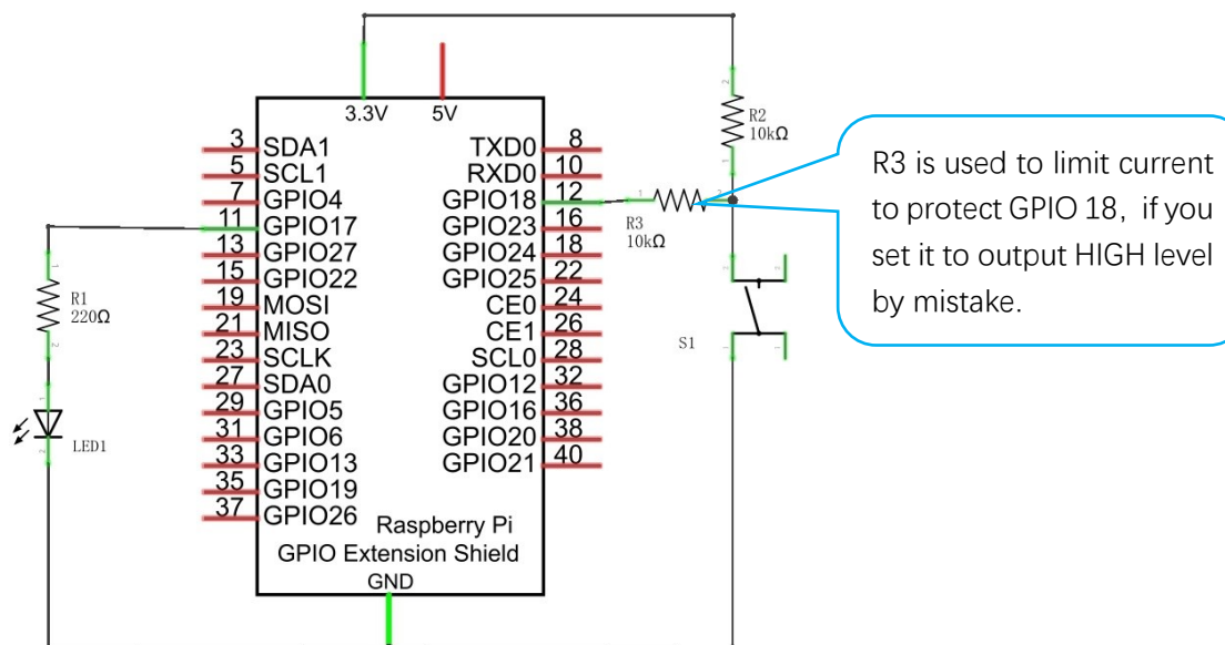
Schematic diagram
