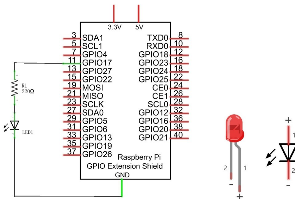
Hardware connection.
