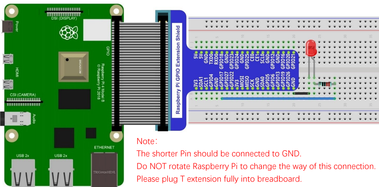
Hardware connection.
