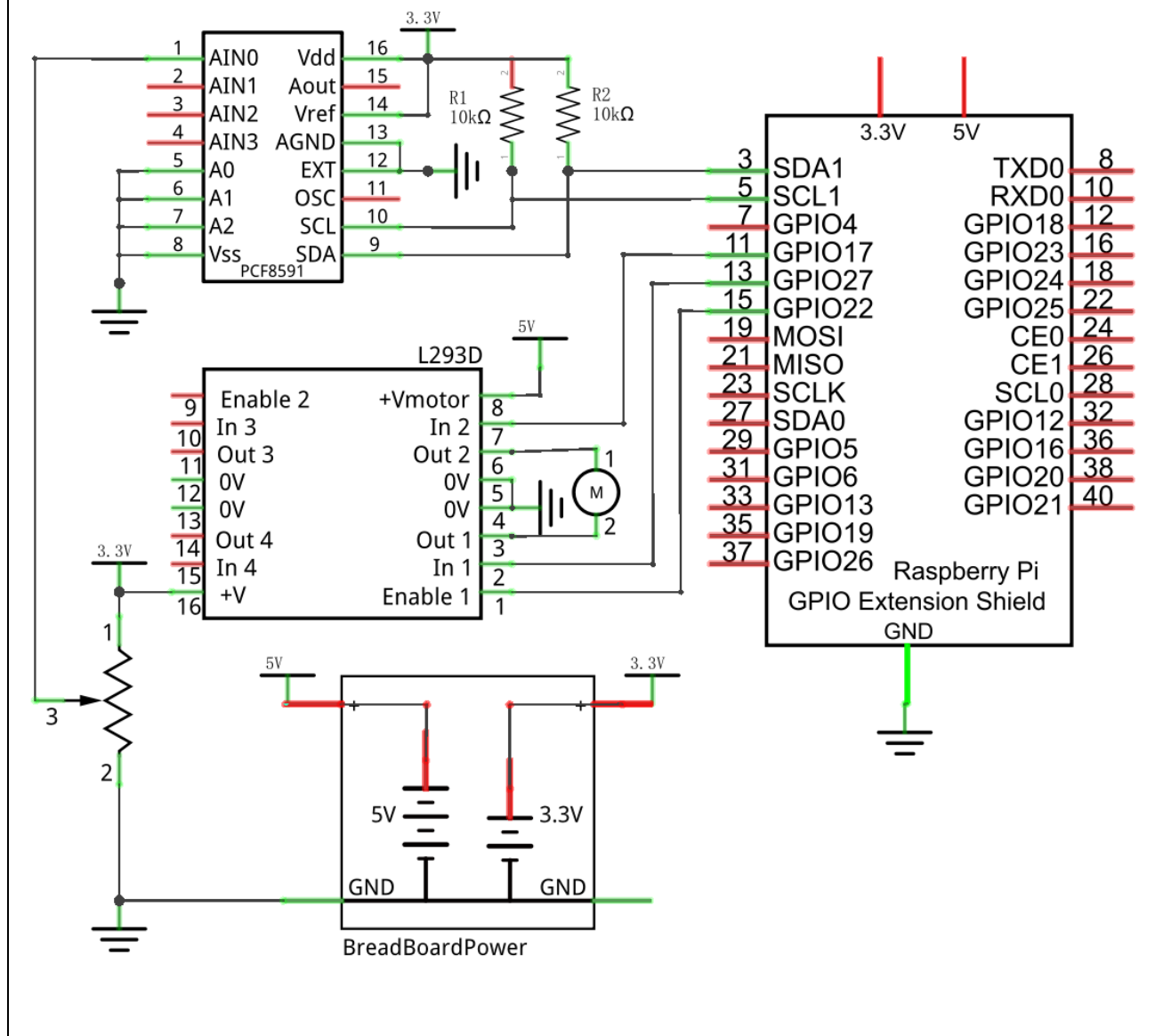
Schematic diagram
