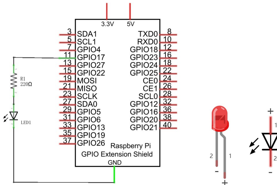
Schematic diagram
