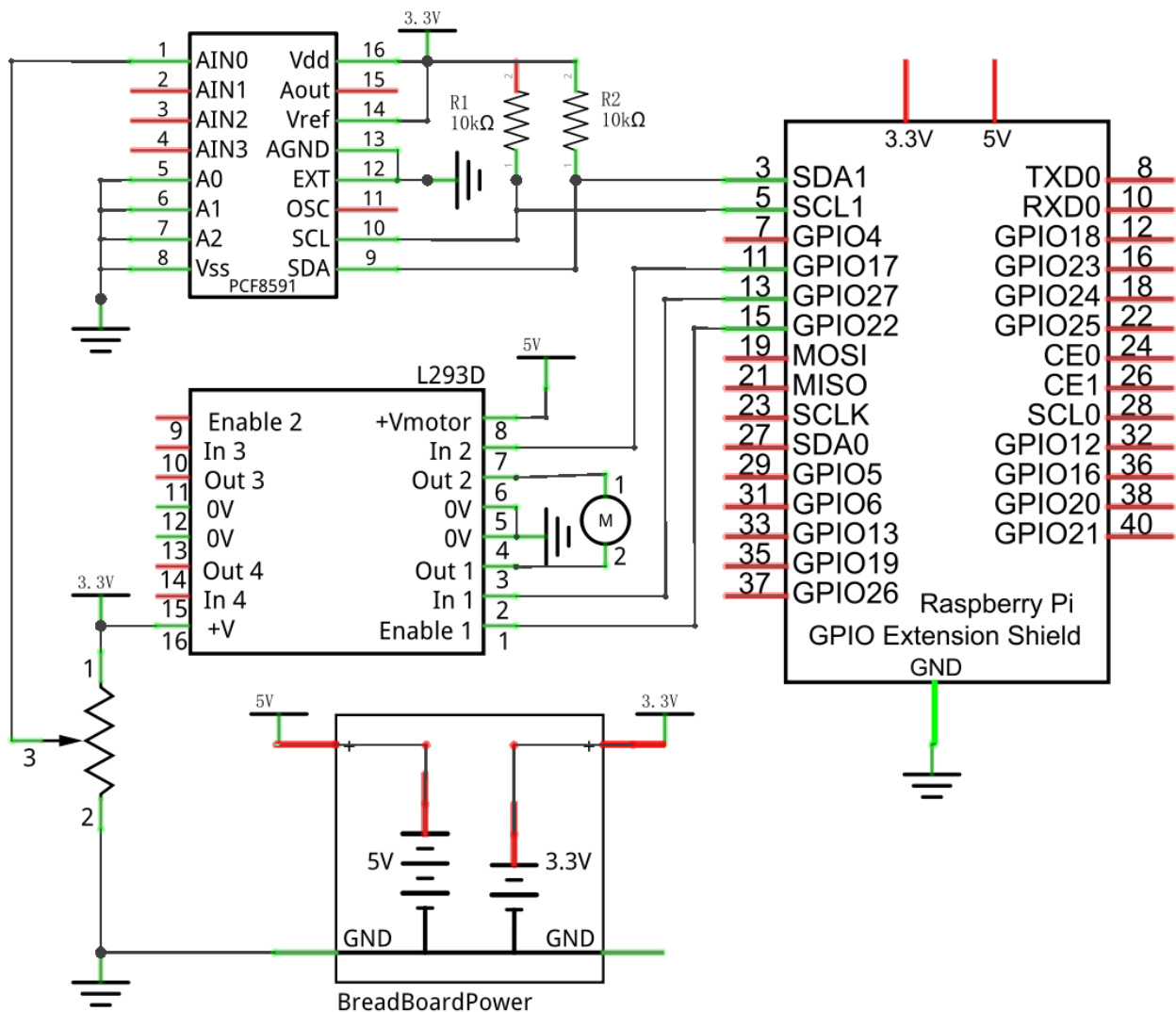
Schematic diagram
