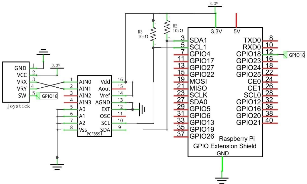
Hardware connection
