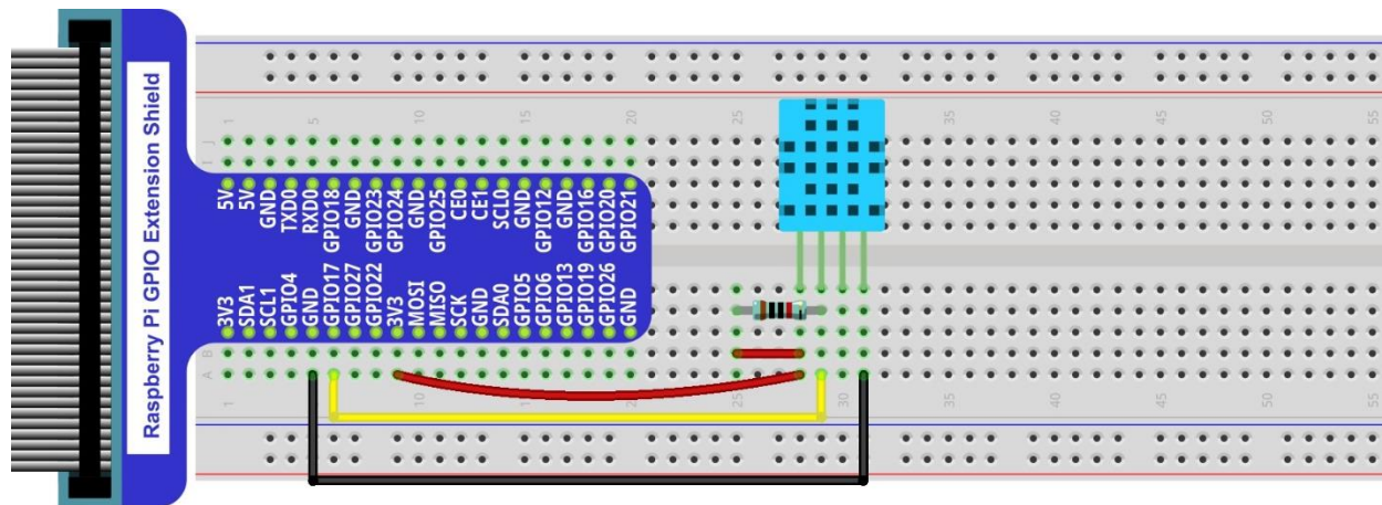
Hardware connection
