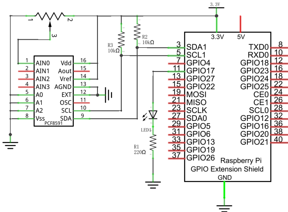
Hardware connection
