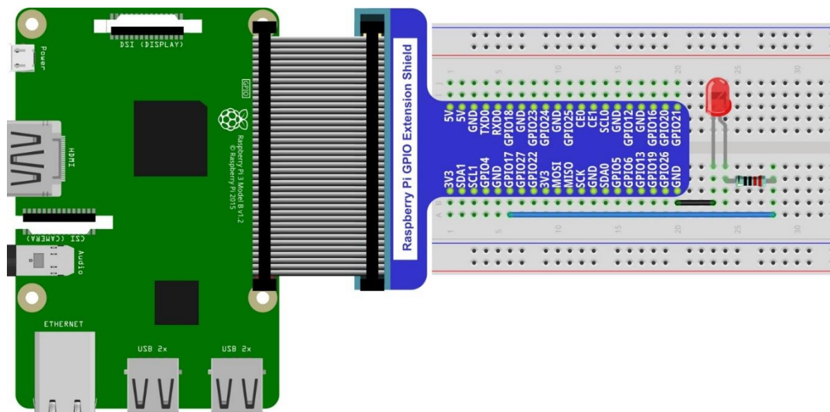
Hardware connection
