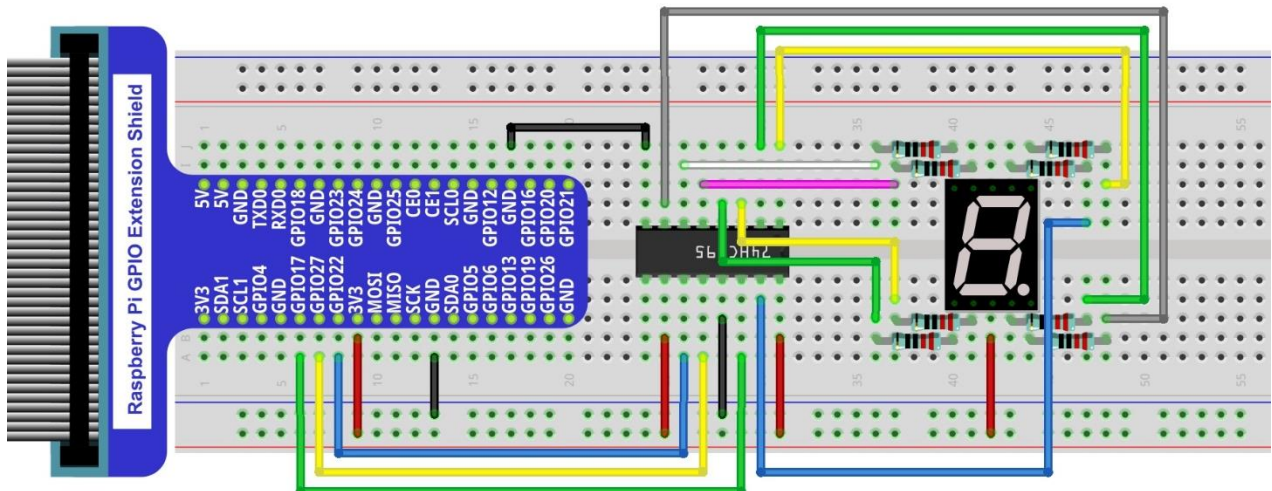
Hardware connection
