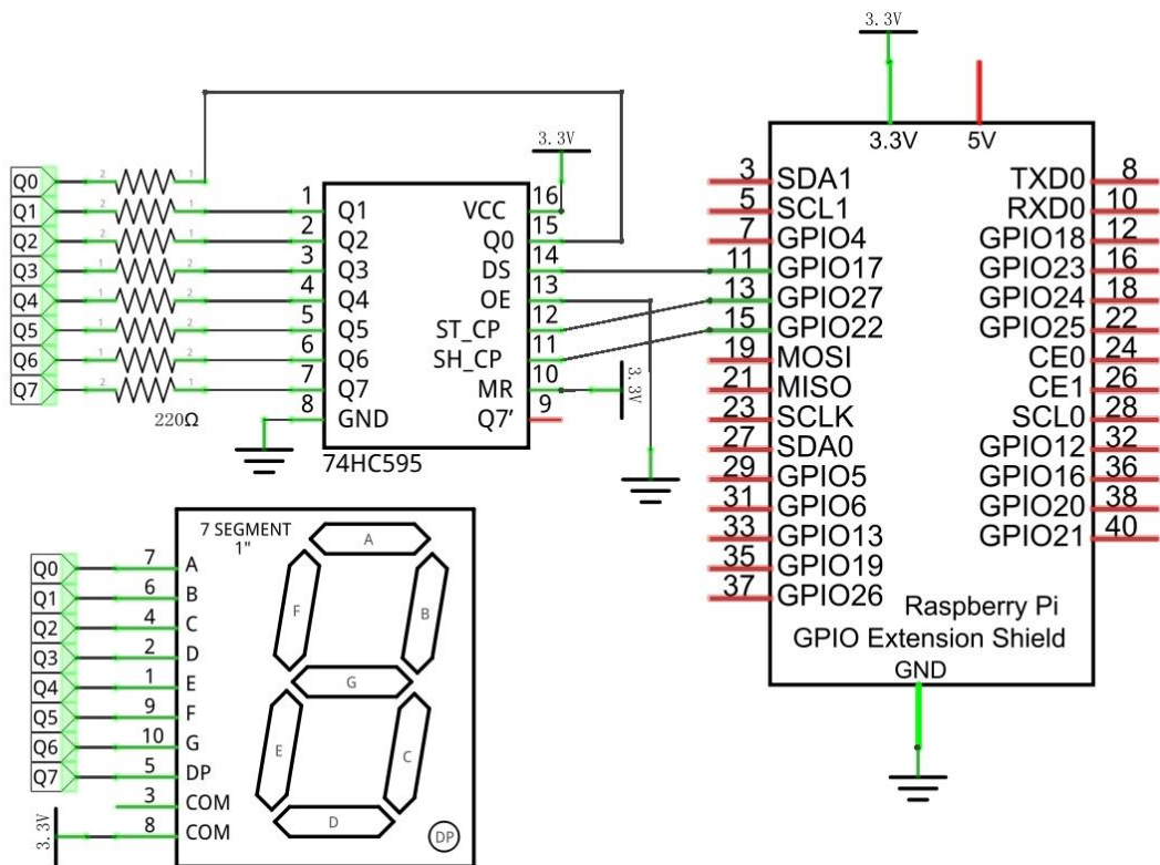
Hardware connection
