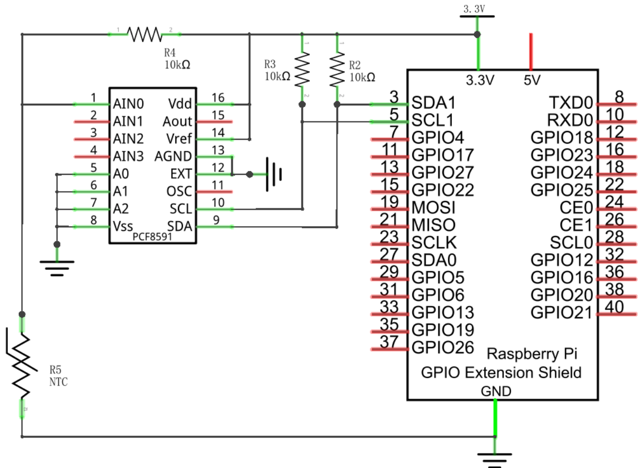
Hardware connection
