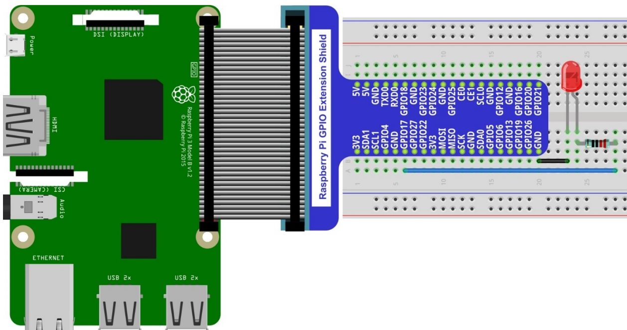
Hardware connection
