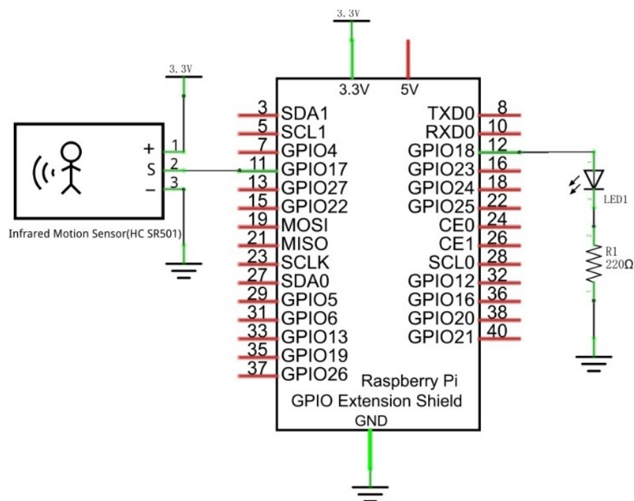
Hardware connection
