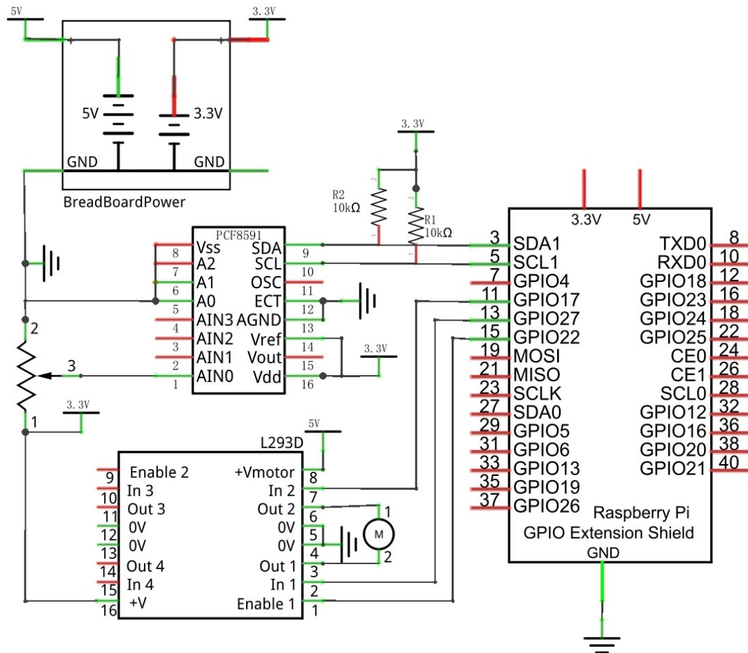
Schematic diagram
