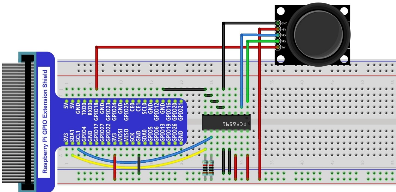
Hardware connection
