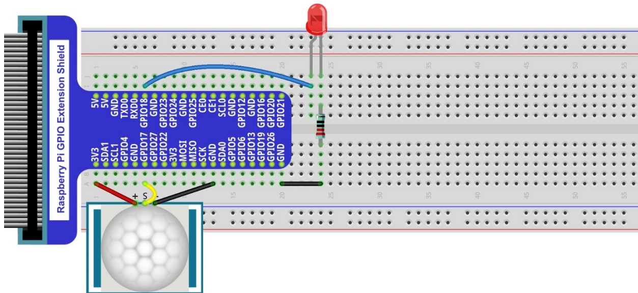
Hardware connection
