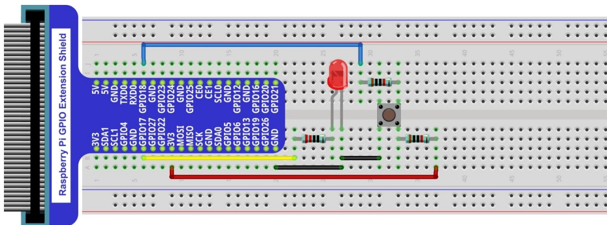
Hardware connection
