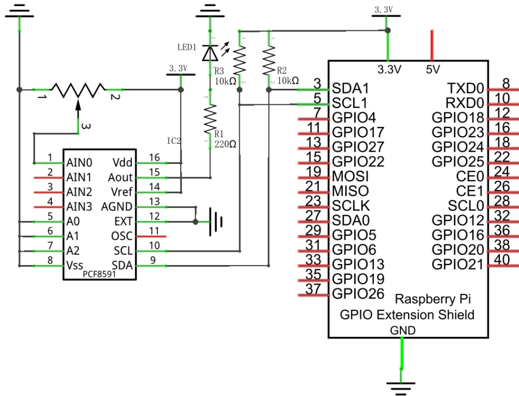
Schematic diagram
