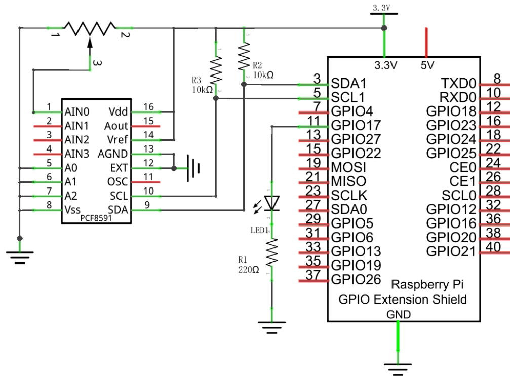
Schematic diagram
