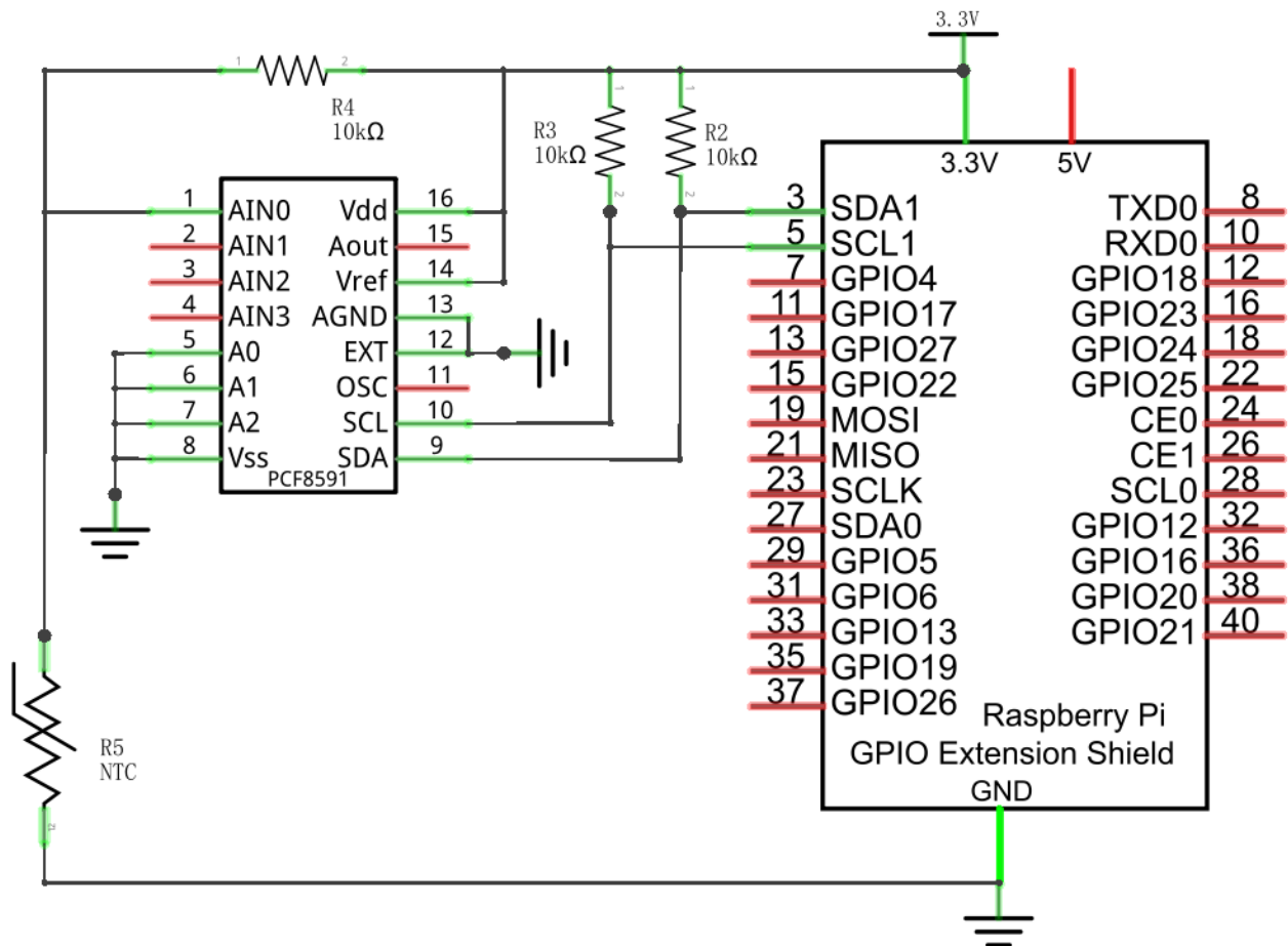
Schematic diagram
