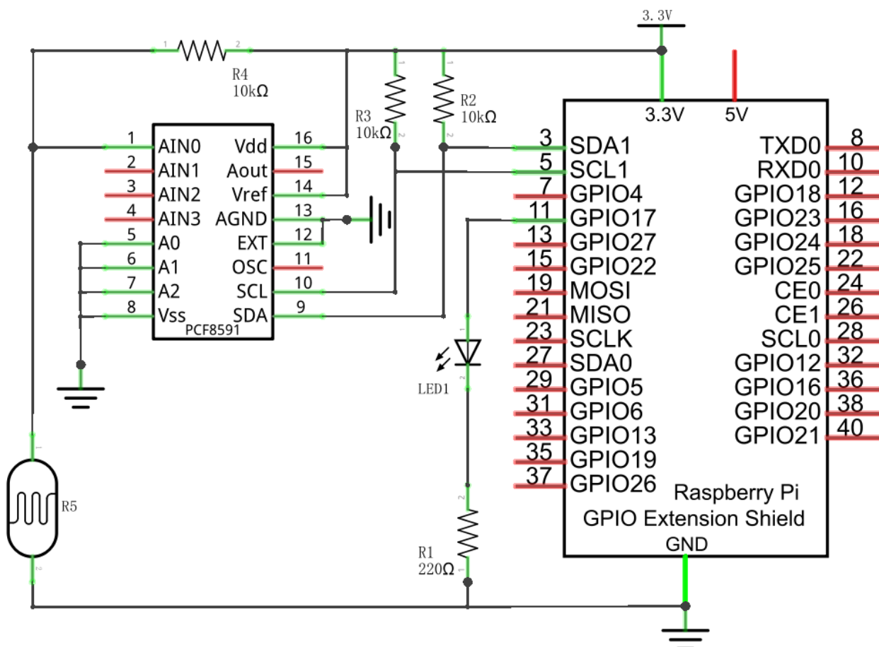
Schematic diagram
