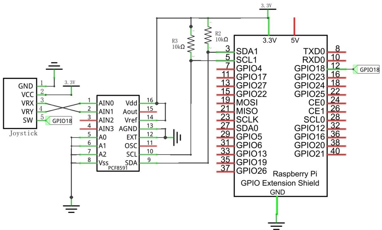
Schematic diagram
