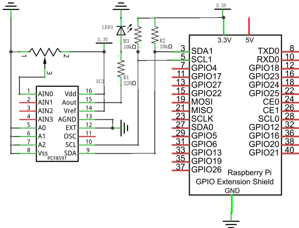
Schematic diagram
