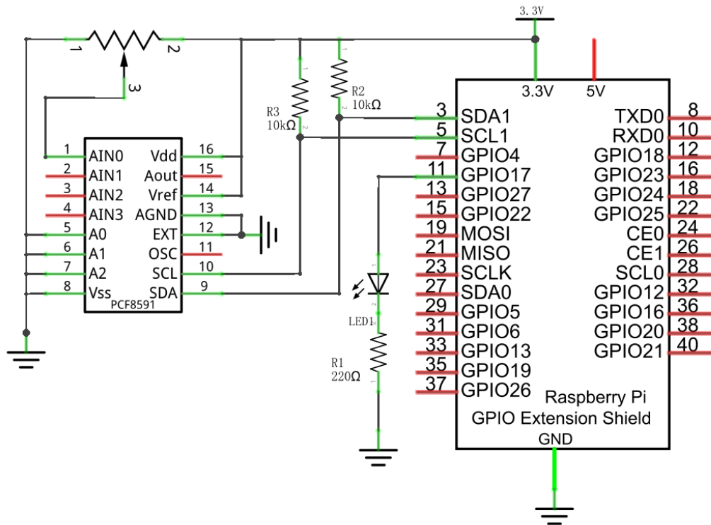
Schematic diagram
