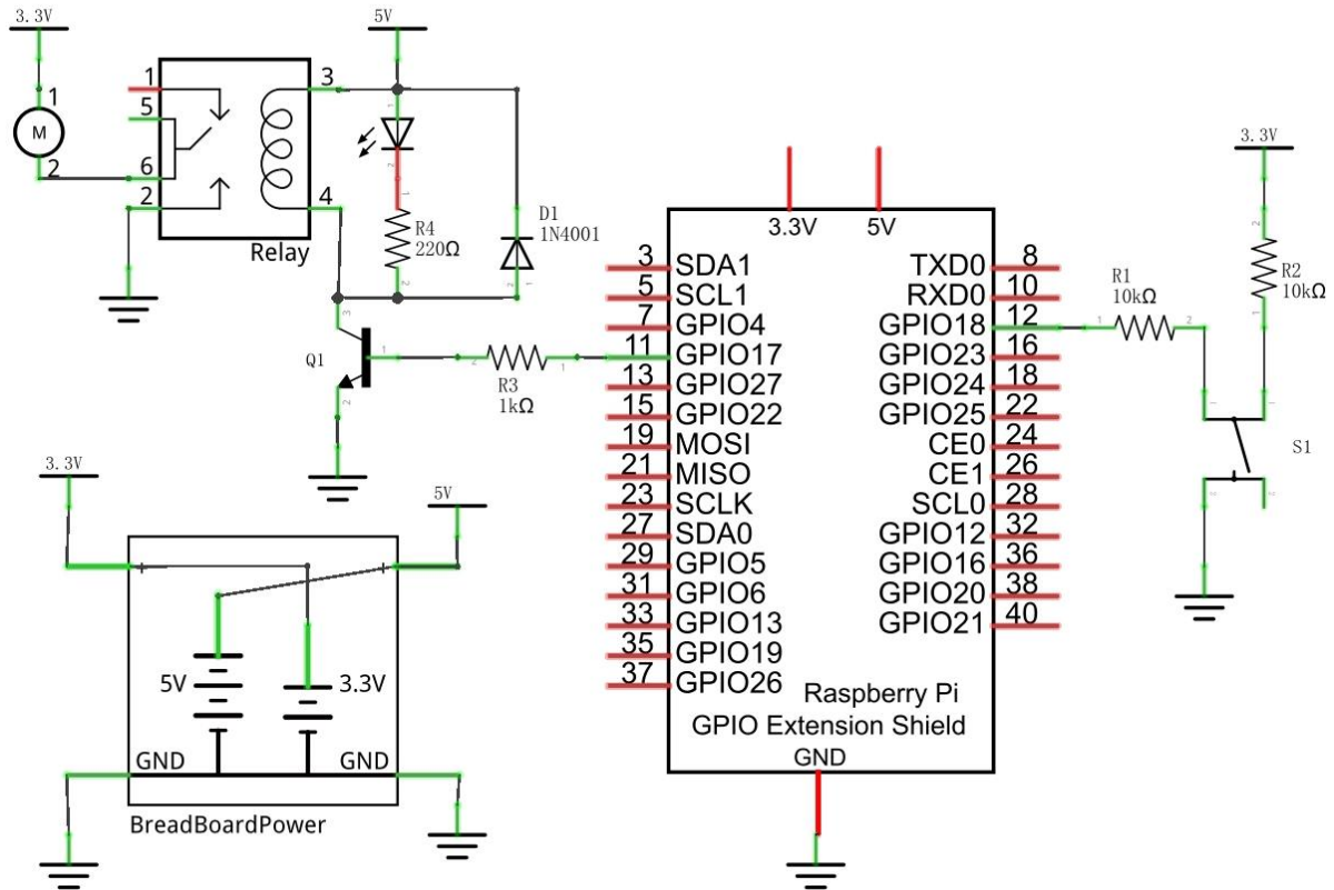
Schematic diagram
