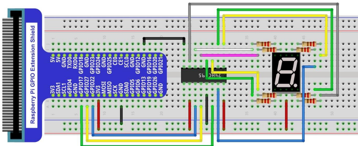
Hardware connection
