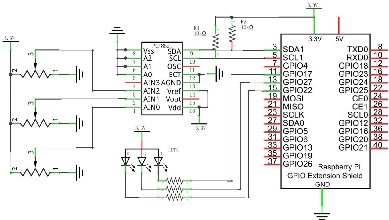
Schematic diagram
