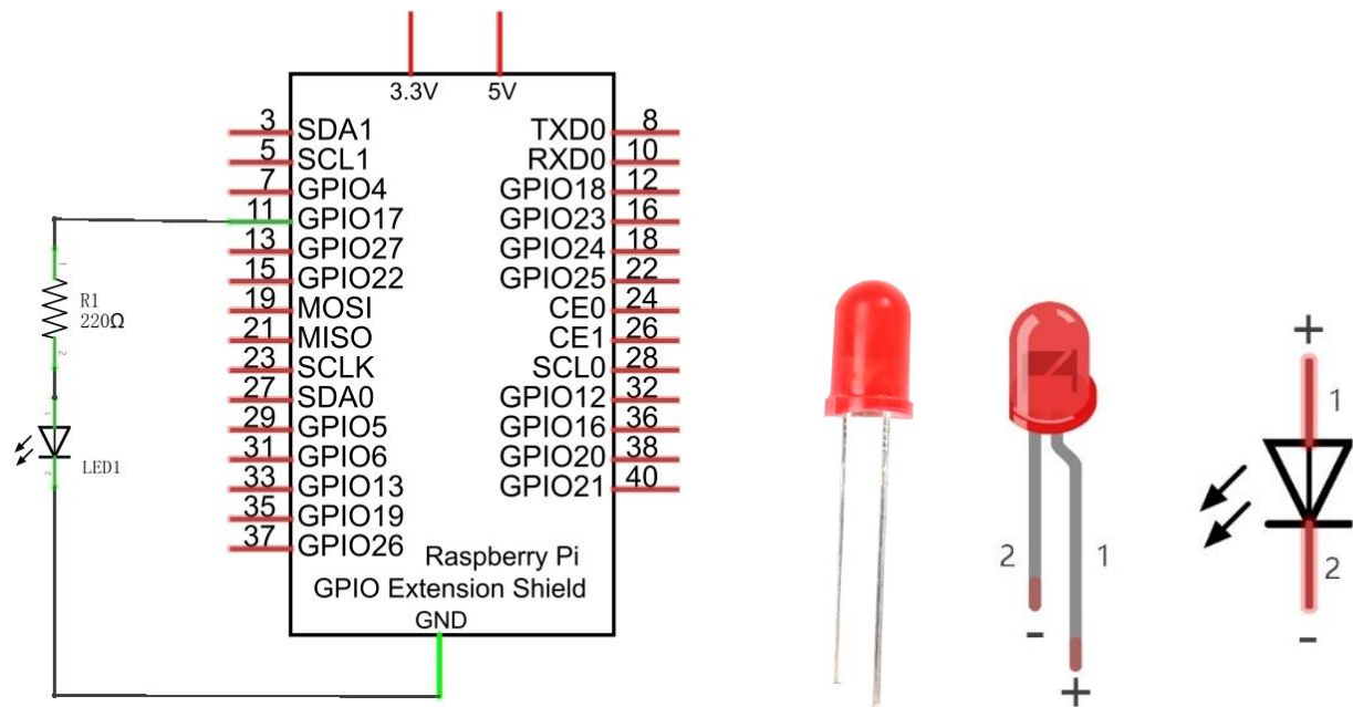
Hardware connection.
