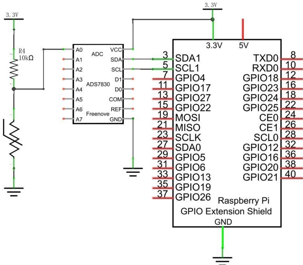
Schematic diagram
