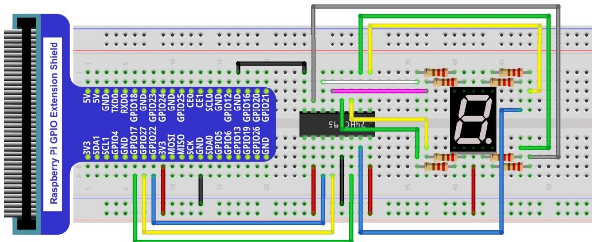
Hardware connection
