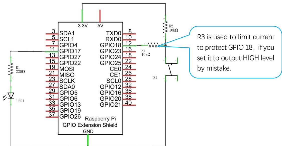
Schematic diagram
