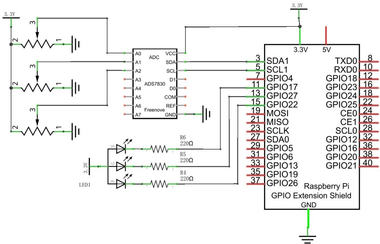
Schematic diagram
