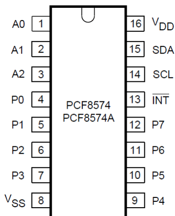
PCF8574 chip pin diagram:
