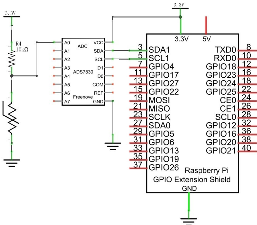
Schematic diagram
