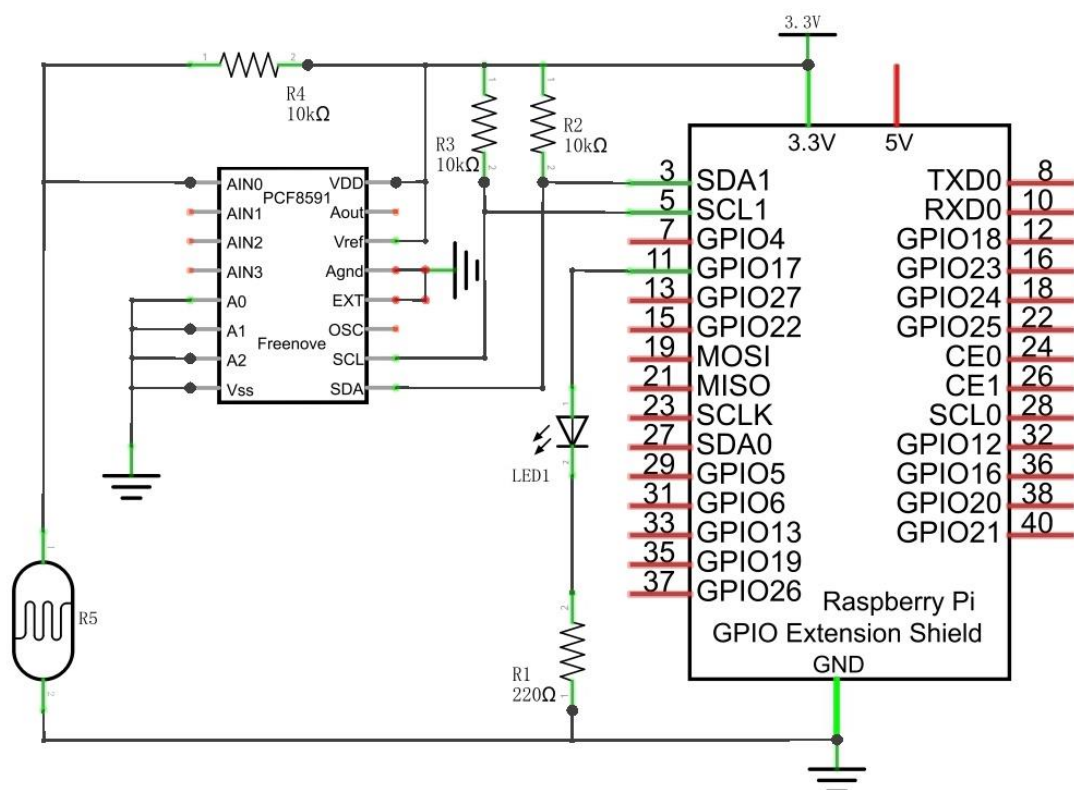
Hardware connection
