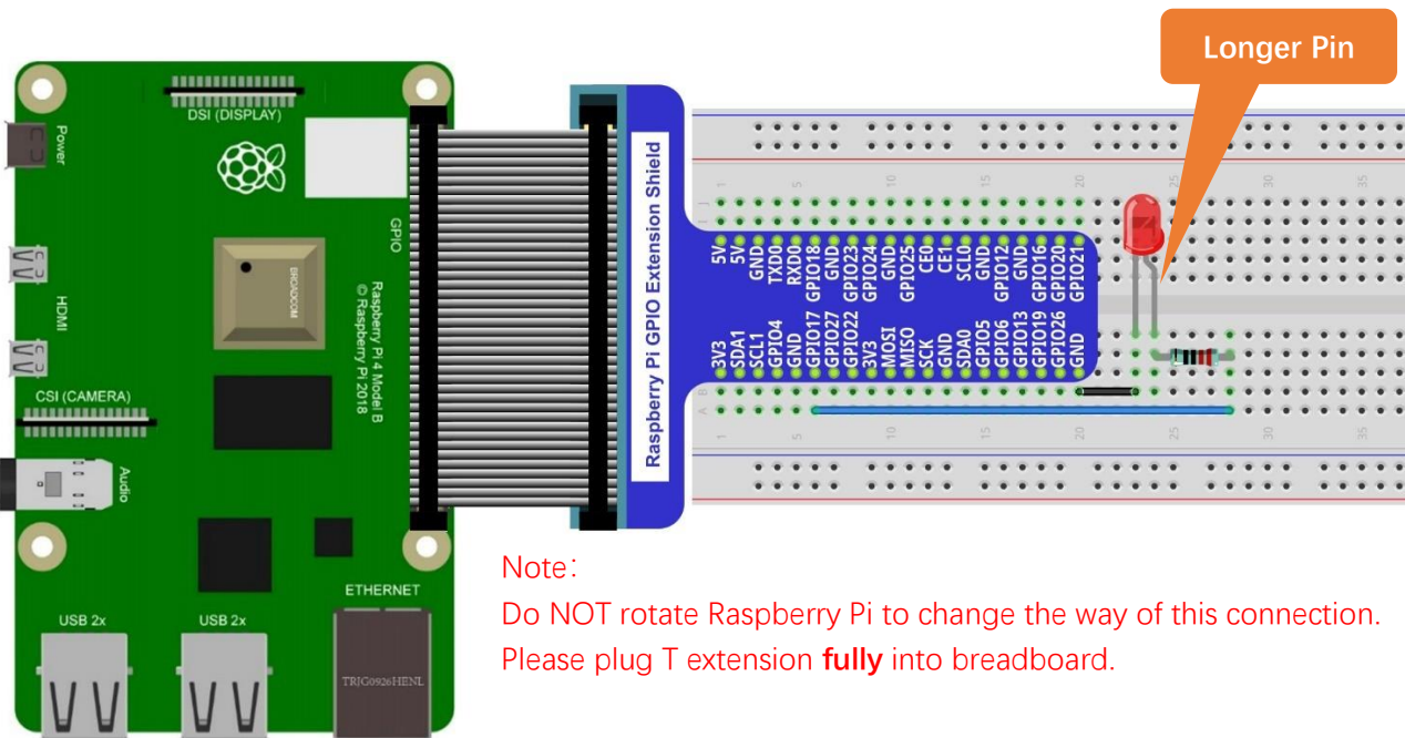
Hardware connection.
