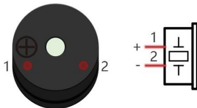
Active buzzer
