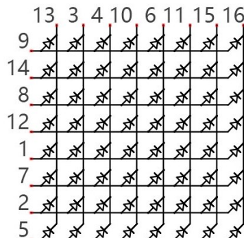
Connection mode of common anode
