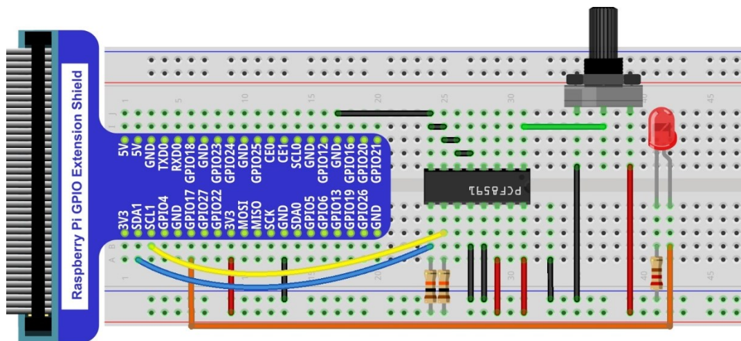
Hardware connection
