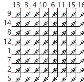
Connection mode of common cathode
