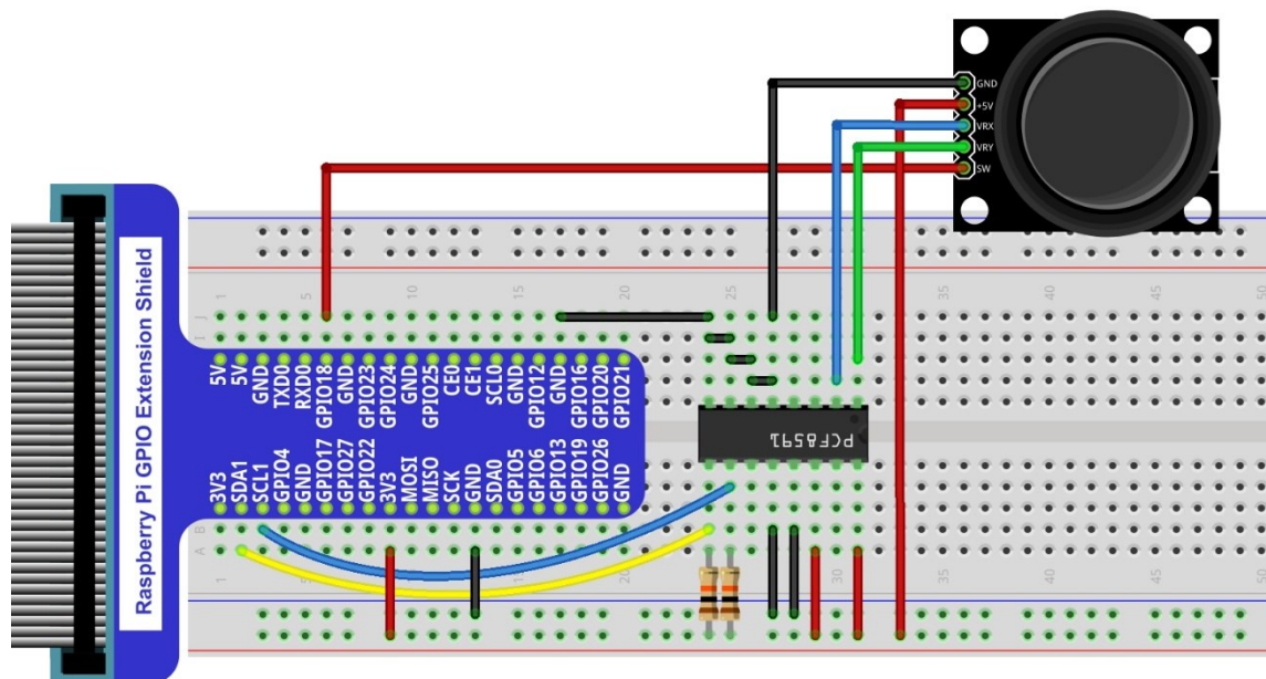
Hardware connection
