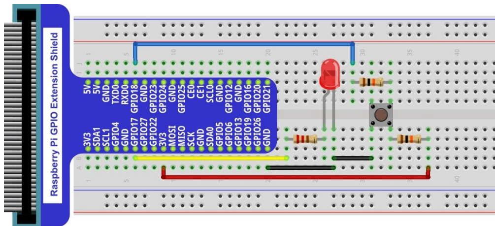
Hardware connection
